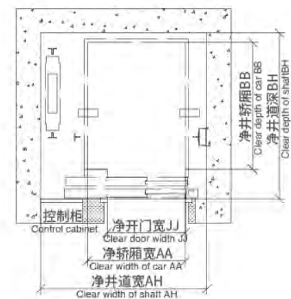
井道平面图(旁开) Shaft layout (side opening)
