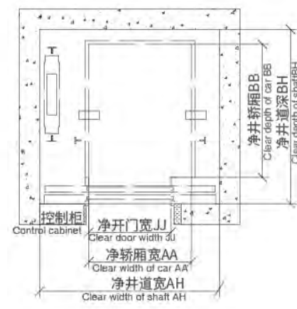
井道平面图(中分) Shaft layout (center opening)
