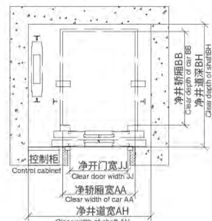
井道平面图(中分双折式) Shaft layout (center opening & double-folded type)
